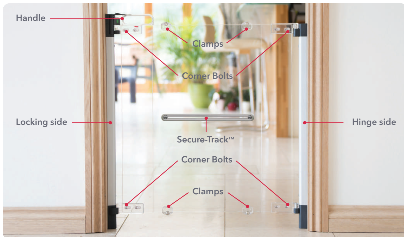
(R) 1 x Screw Fit Clear-View Gate
